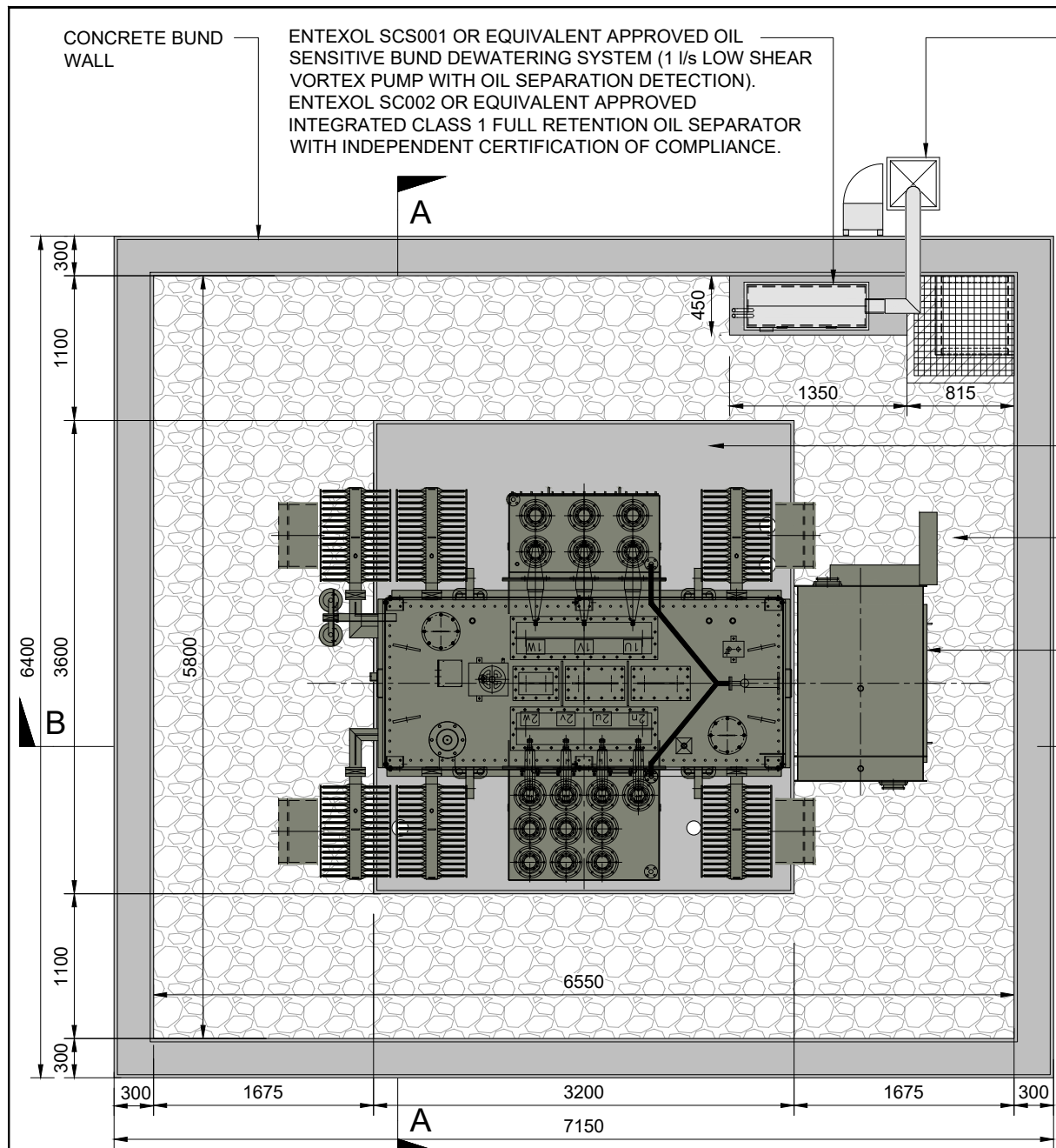
TRANSFORMER BUND PLAN SCALE 1:50
